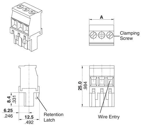
Right-Hand Version
