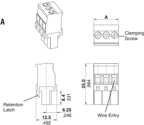
Left-Hand Version
