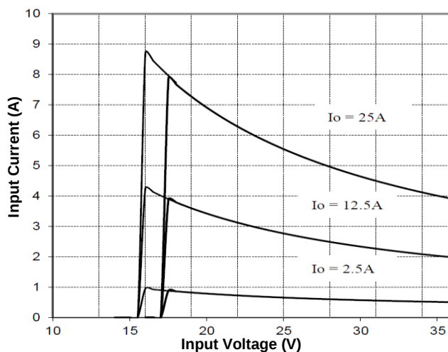
Figure 9. Input Characteristics
