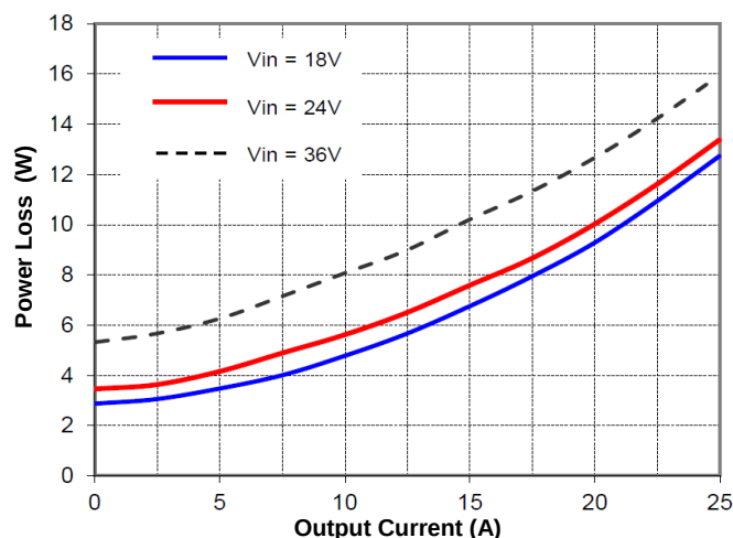
Figure 2. Power Loss vs. Load Current (25°C)
