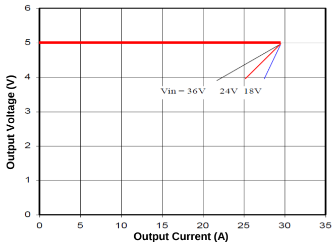
Figure 10. Output Characteristics
