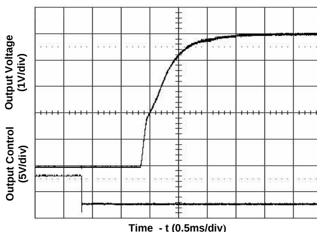
Figure 4. Start-Up from Enable Control Input voltage 24V, Output current 0A
