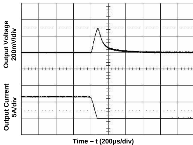
Figure 7. Transient Load Response
