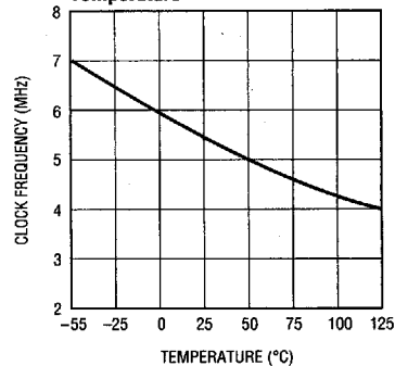
Maximum Clock Frequency vs Temperature
