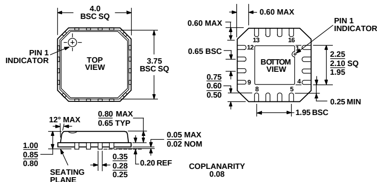
Figure 64. 16-Lead Lead Frame Chip Scale Package [LFCSP] 4 mm x 4 mm Body (CP-16)
