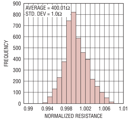
Normalized Input 400 \Omega Resistor Trim
