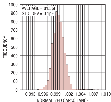
Normalized 81.5pF Capacitor Trim
