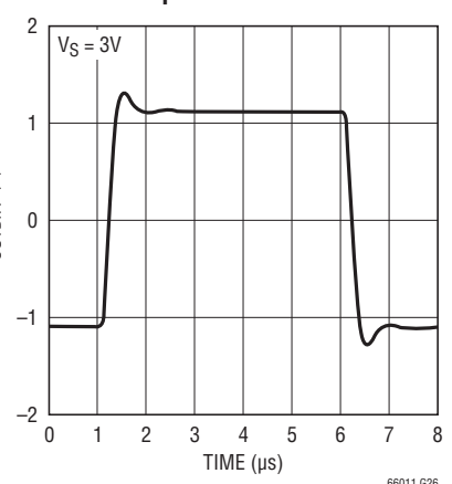
Pulse Response
