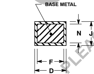
SECTION AE-AE
