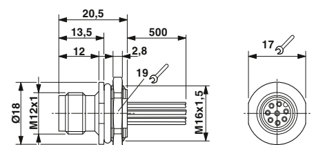
M12 pin, M16 fastening thread
