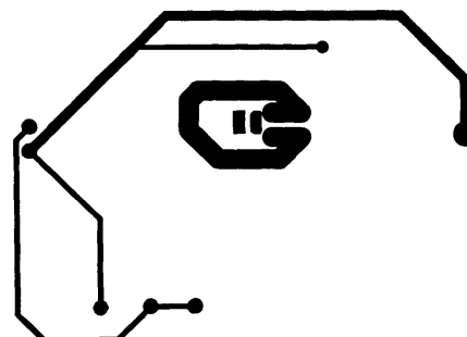
Figure 59. Recommended 20-pin DSBGA PC Board Layout: Lower Inner-Layer Layout
