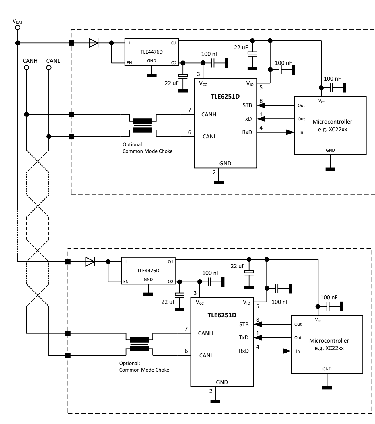
Figure 13 Application circuit
