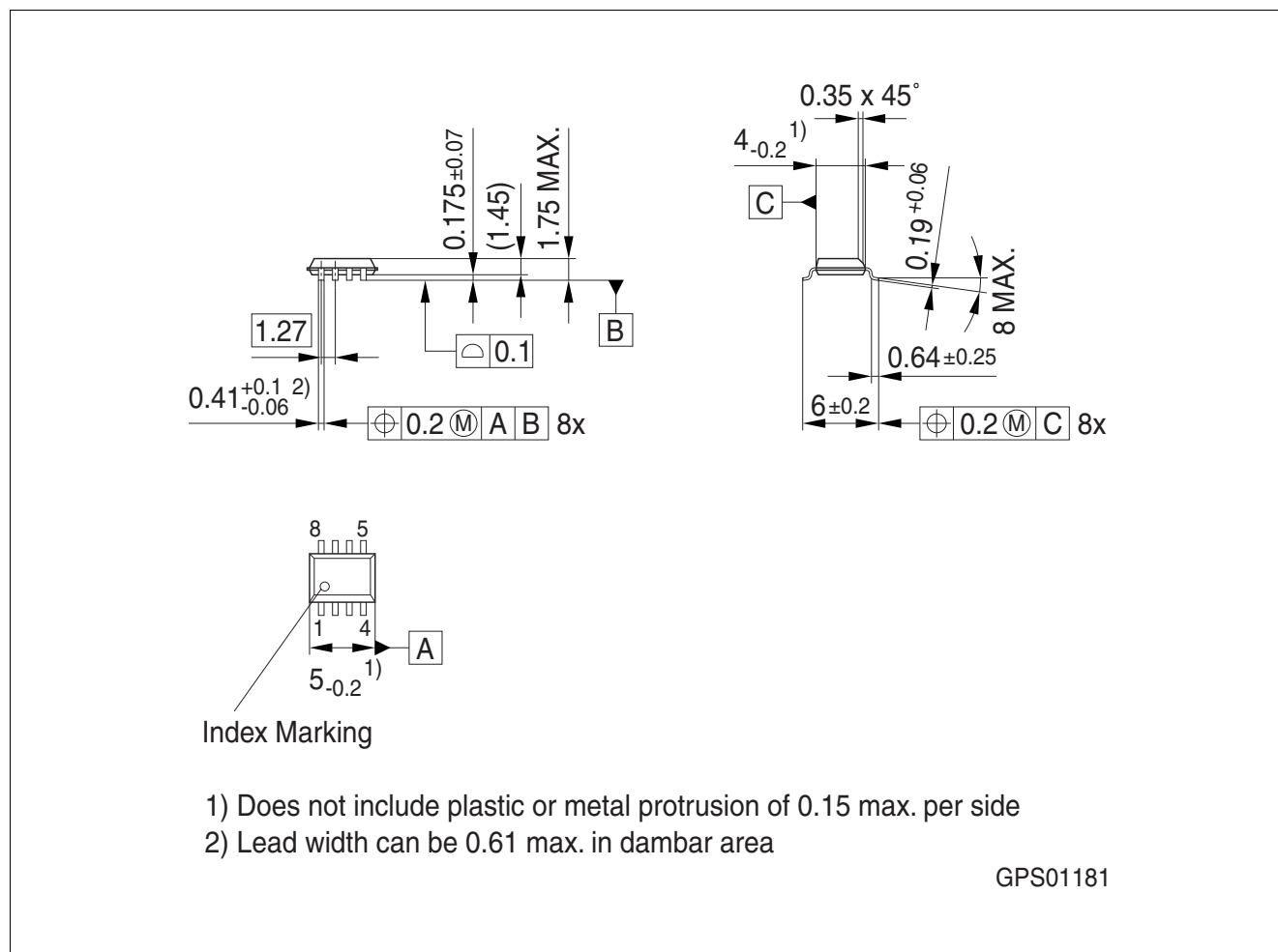
Figure 14 PG-DSO-8 (Plastic Dual Small Outline)
