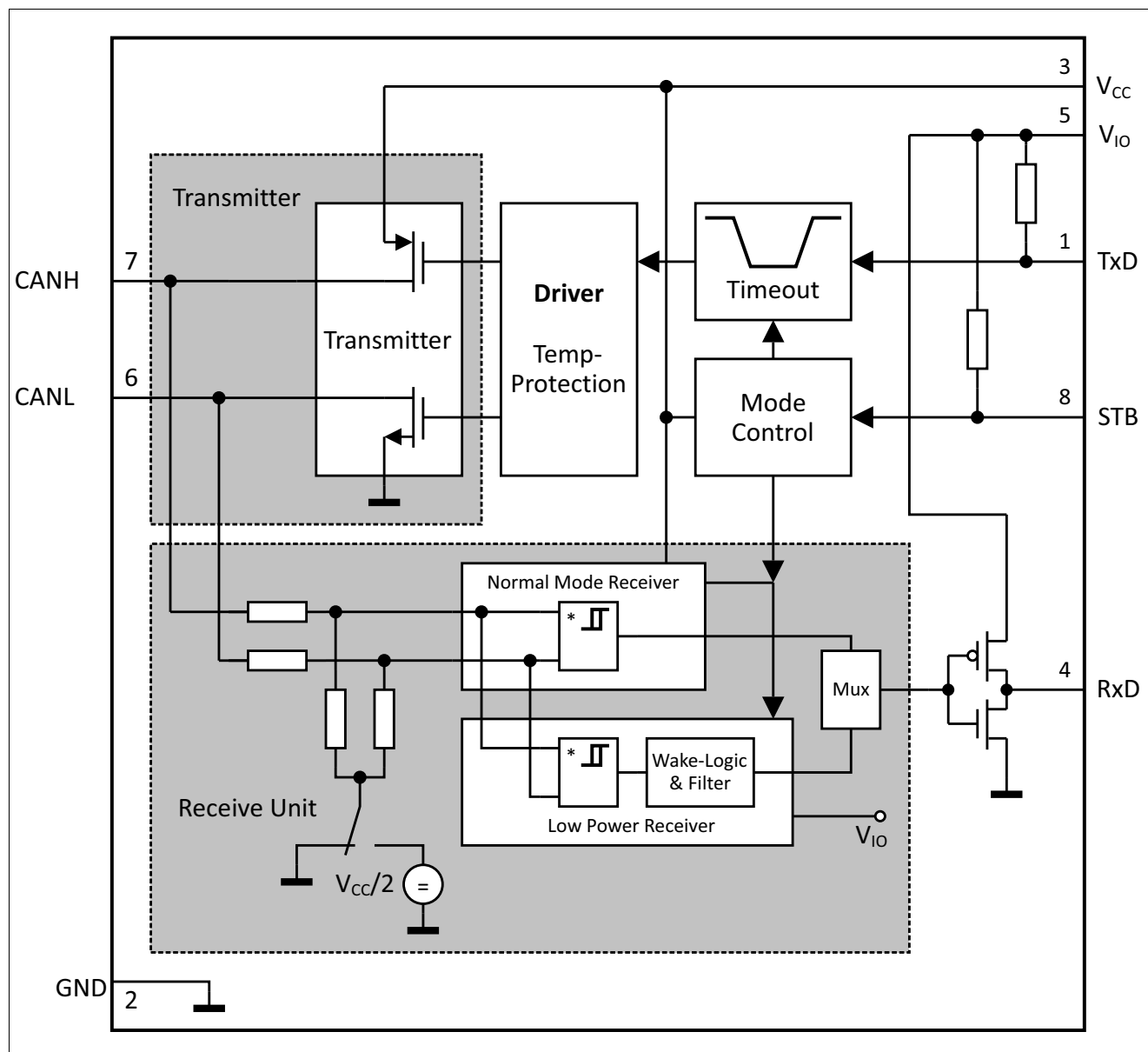
Figure 1 Block diagram
