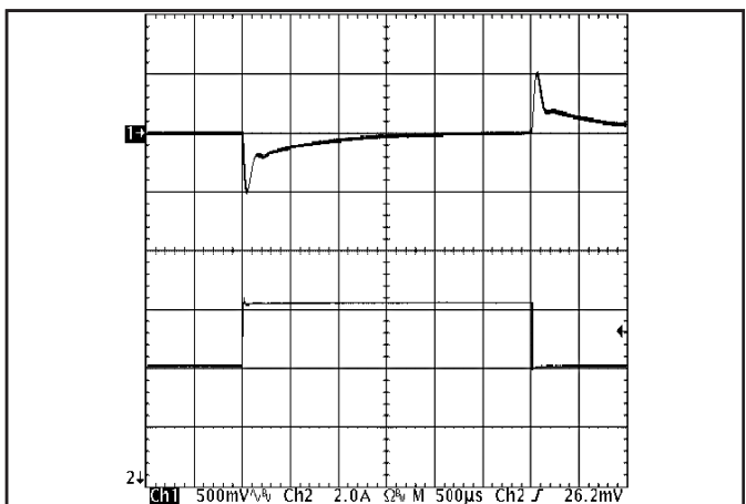
Figure 12: Output voltage response to step-change in load current (50%-75%-50% of I_{out(max)} ; dI/dt = 5\text{A}/\mu\text{s} ). Load cap: 100μF, 30 mΩ ESR tantalum capacitor and 1μF ceramic cap. Ch 1: V_{out} (500mV/div), Ch 2: I_{out} (2A/div).
