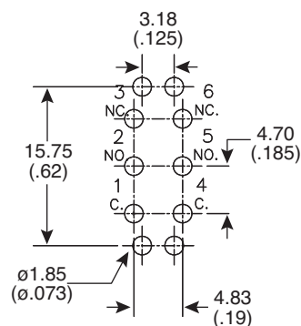
P.C. MOUNTING
