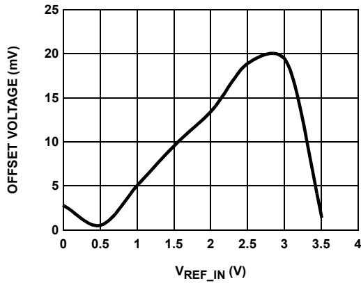
FIGURE 17. DC OFFSET VOLTAGE AT V OUT vs V REF_IN
