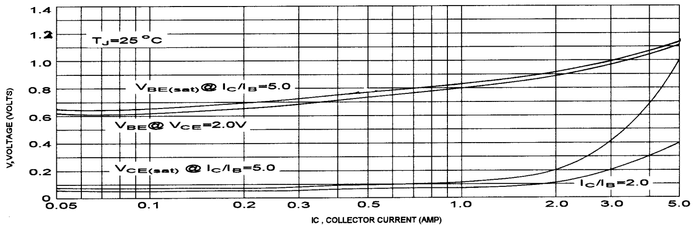
"ON" VOLTAGES
