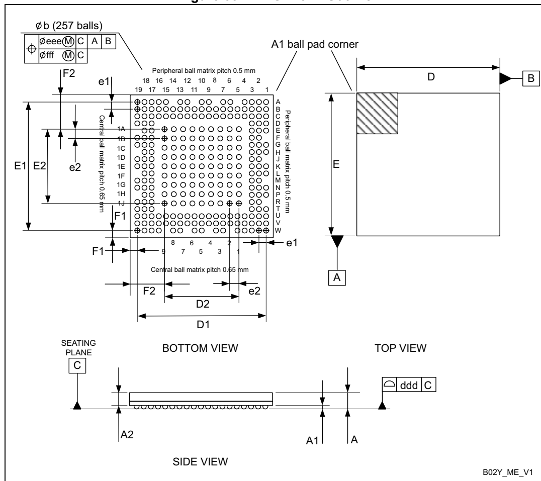
Figure 66. TFBGA257 - Outline
