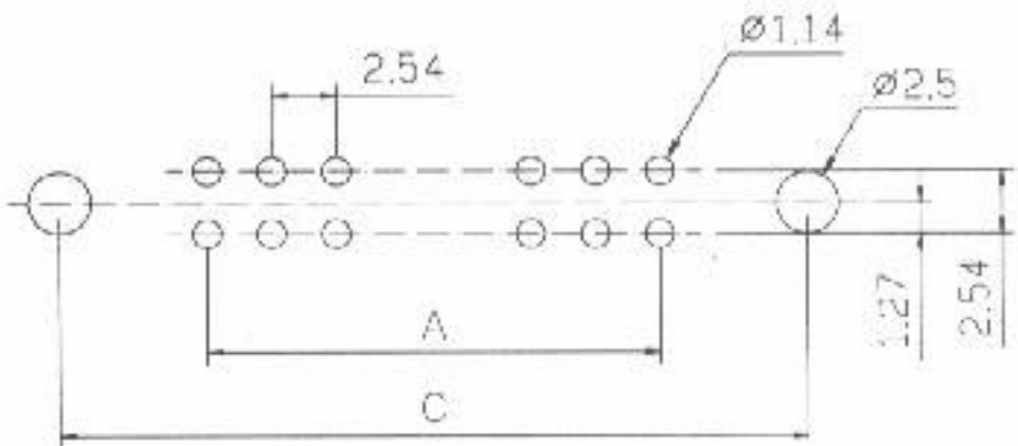
Recommend PCB Layout
