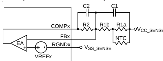
Figure 10. Loop Setting with Temperature Compensation
