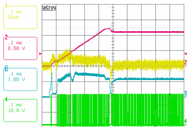
FIGURE 29. SOFT START IN-RUSH CURRENT, V_{IN} = 19V , I_O = 2A , V_{ID} = 1.1V , Ch1: DR00P-V0 (2.1mV = 1A), Ch2: V_O , Ch3: V_{COMP} , Ch4: PHASE
