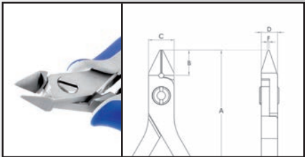
Cutting capacity wire mm/AWG
