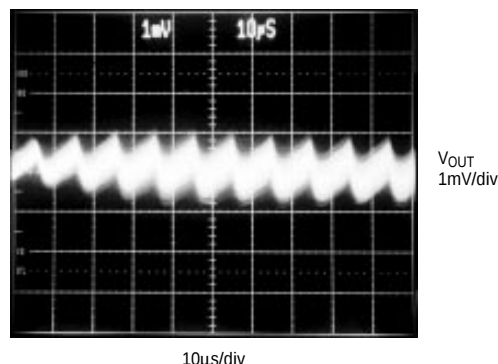
MAX840 OUTPUT NOISE AND RIPPLE ( C_1 = C_2 = C_3 = 0.22\mu F , C_4 = 4.7\mu F )
