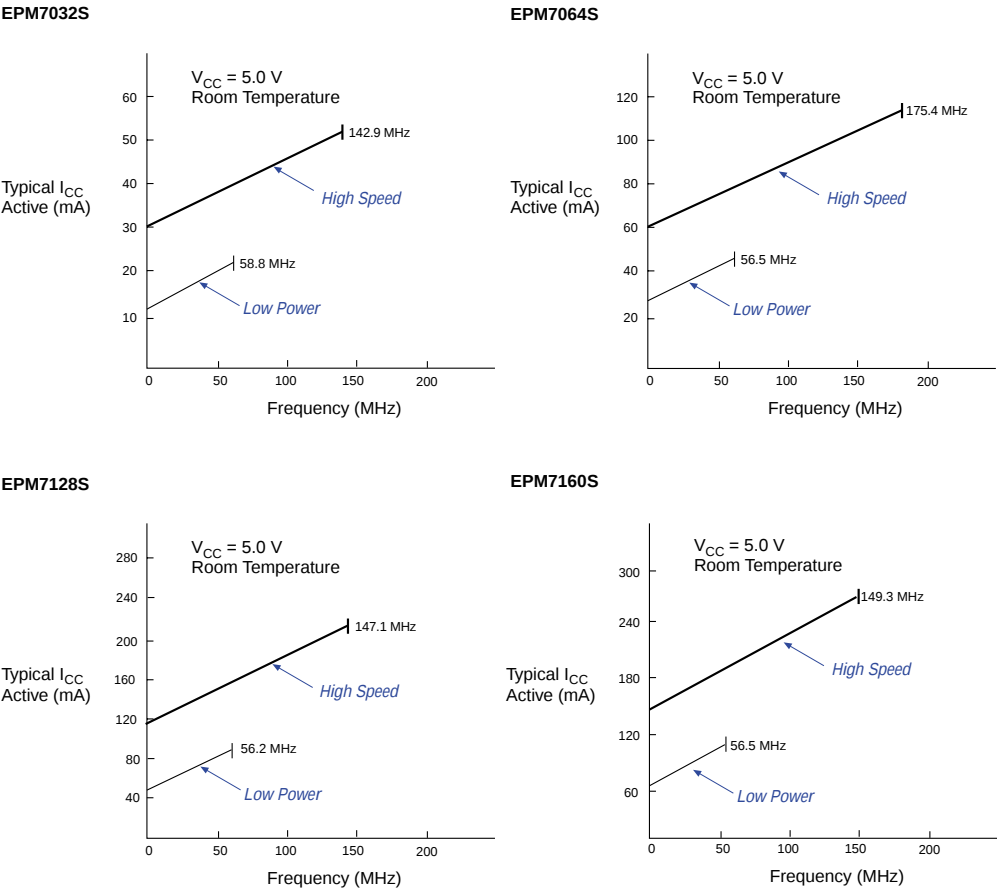
Figure 15. I_{CC} vs. Frequency for MAX 7000S Devices (Part 1 of 2)
