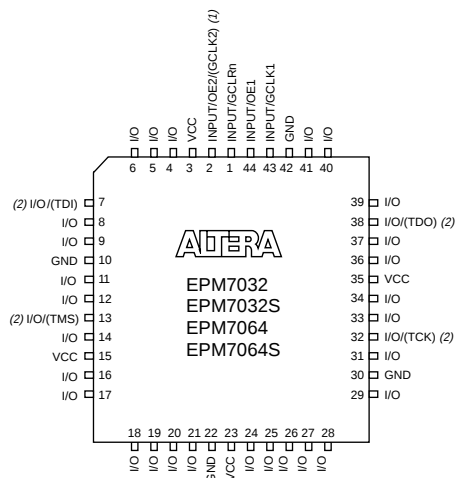
44-Pin PLCC
