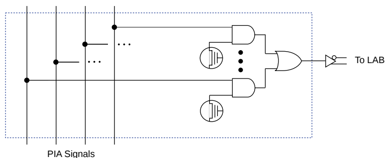
Figure 7. PIA Routing
