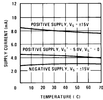
Supply Currents
