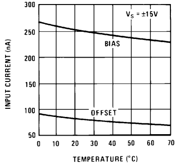
Input Currents
