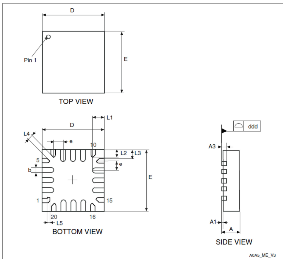
20-lead ultra thin fine pitch quad flat no-lead package outline (3x3)*
