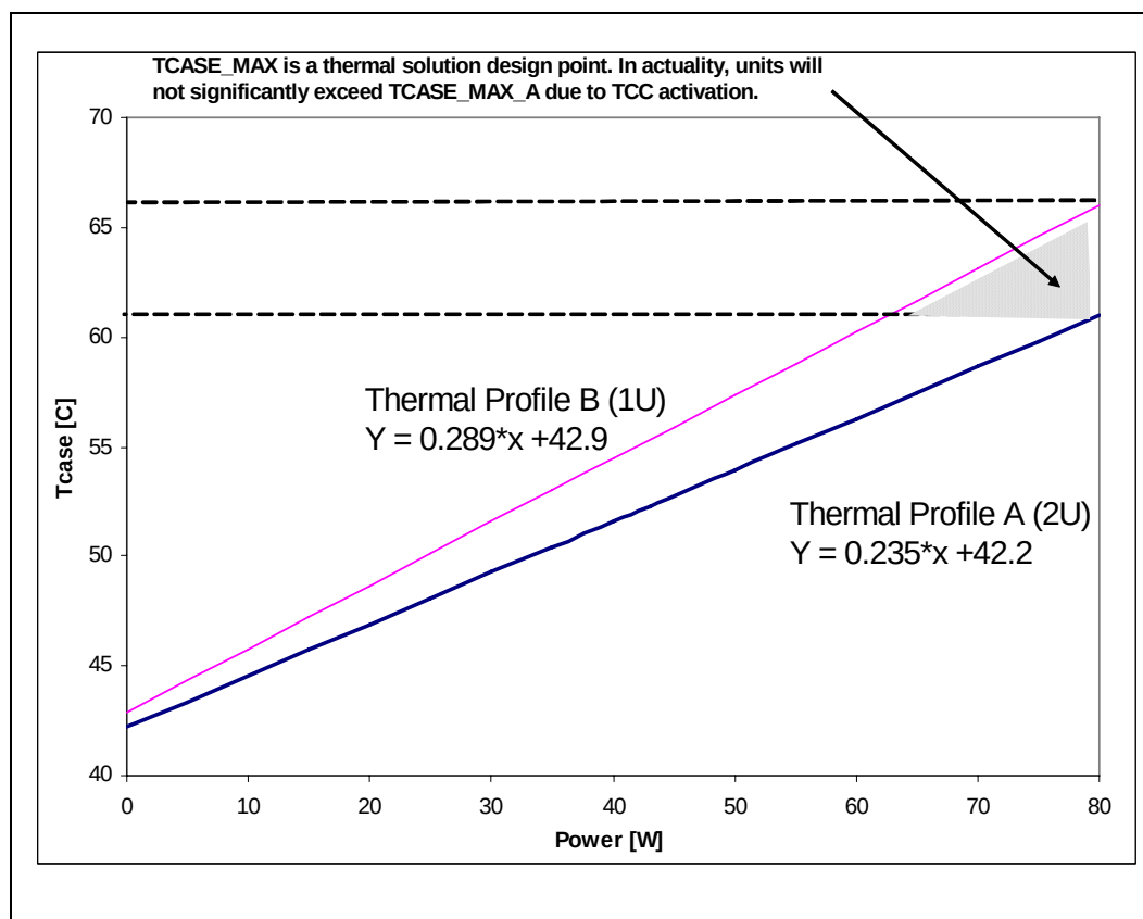
Figure 6-2. Dual-Core Intel® Xeon® Processor X5200 Series Thermal Profiles A and B
