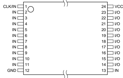
TSSOP Top View
