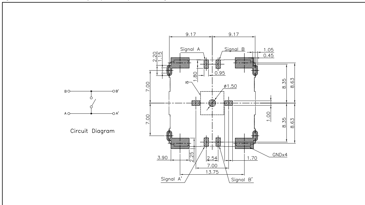
Figure 6. Recommended PCB Layout (mm \pm 0.05 ) & Circuit Diagram
