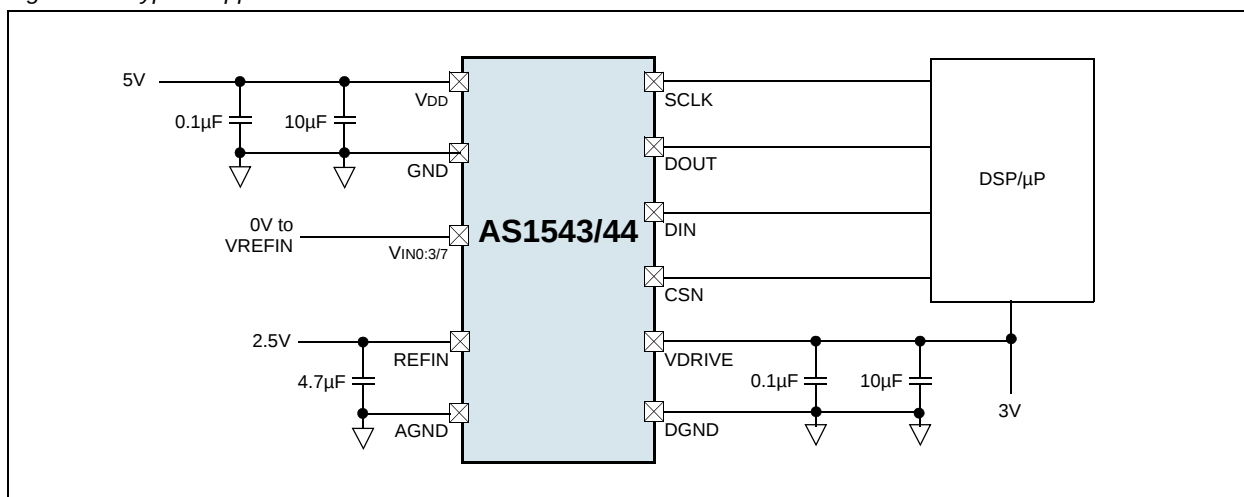
Figure 35. Typical Application
