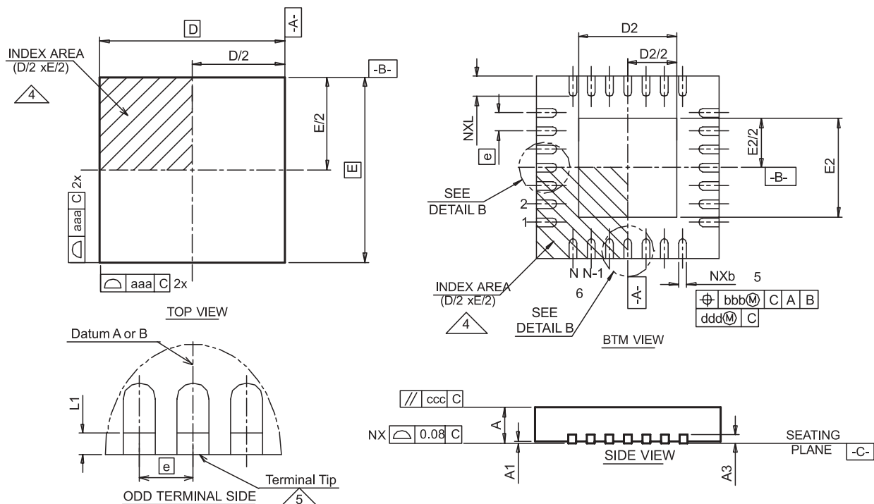
Figure 36. TQFN(4x4)-20 Package
