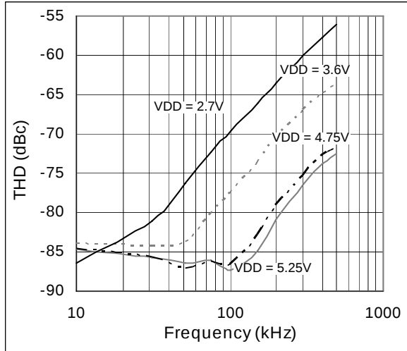
Figure 11. THD vs. Input Signal Frequency
