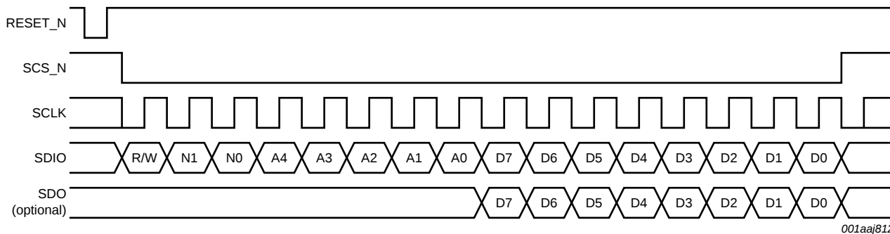
Fig 3. SPI protocol
