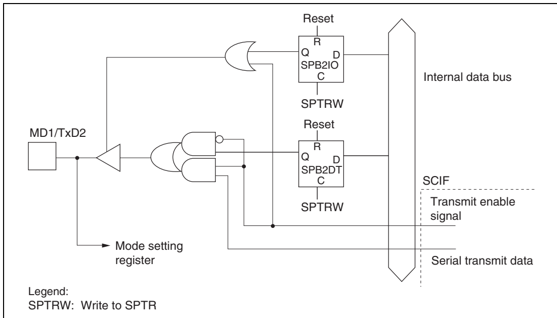
Figure 18.6 MD1/TxD2 Pin
