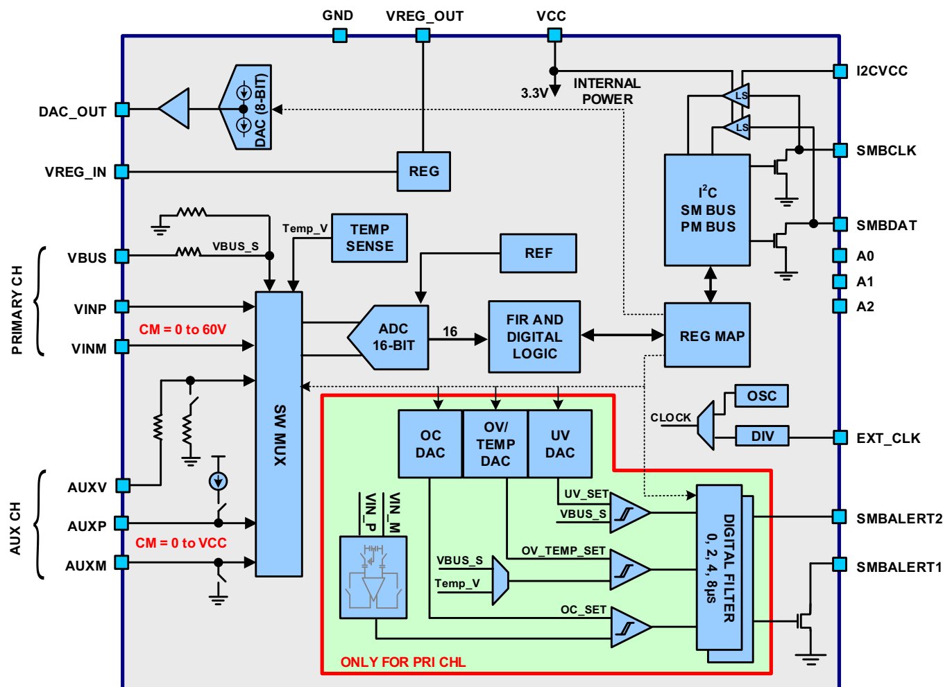
FIGURE 2. BLOCK DIAGRAM
