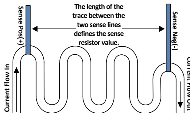
FIGURE 126. ILLUSTRATES A LAYOUT EXAMPLE OF A CURRENT SENSE RESISTOR MADE FROM A PCB TRACE
