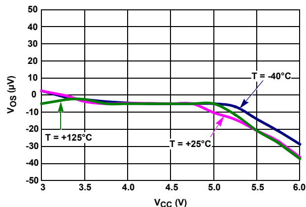
FIGURE 28. AUXILIARY V_{SHUNT} V_{OS} vs V_{CC}
