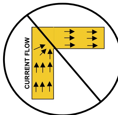
FIGURE 121. AVOID ROUTING ORTHOGONAL CONNECTIONS FOR TRACES THAT HAVE HIGH CURRENT FLOWS
