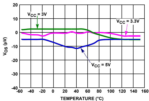
FIGURE 30. AUXILIARY V_{SHUNT} V_{OS} vs TEMPERATURE
