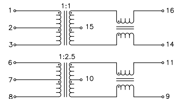
SCHEMATIC - PINS 4, 5, 12 AND 13 NOT CONNECTED
