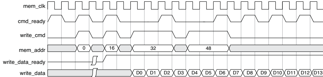
Figure 2-10. Timing Diagram for Memory Write
