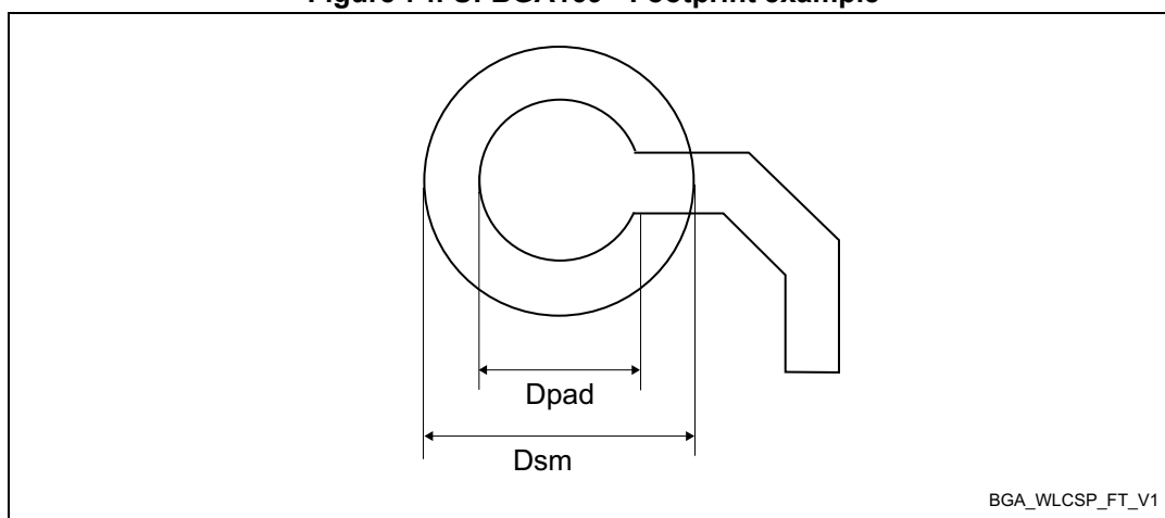
Figure 74. UFBGA169 - Footprint example
