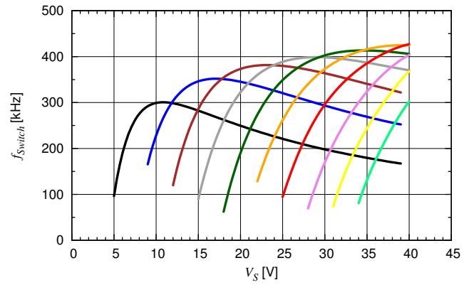
f_{\text{Switch}} versus V_s and Number of LEDs
