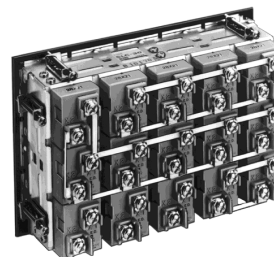
Staggered Terminals: increased safety and serviceability
