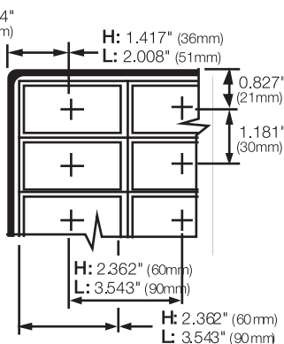
Multiple Windows
