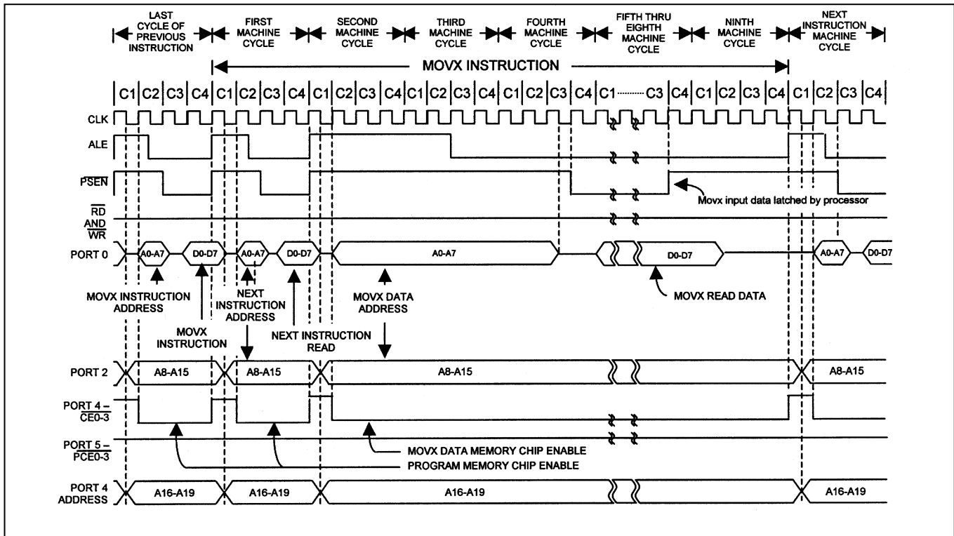
Figure 11. Multiplexed 9-Cycle Data Memory \overline{\text{CE0-3}} Read
