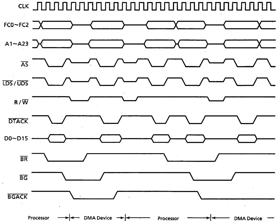
Figure 4.12 Bus Arbitration Cycle Timing Diagram
