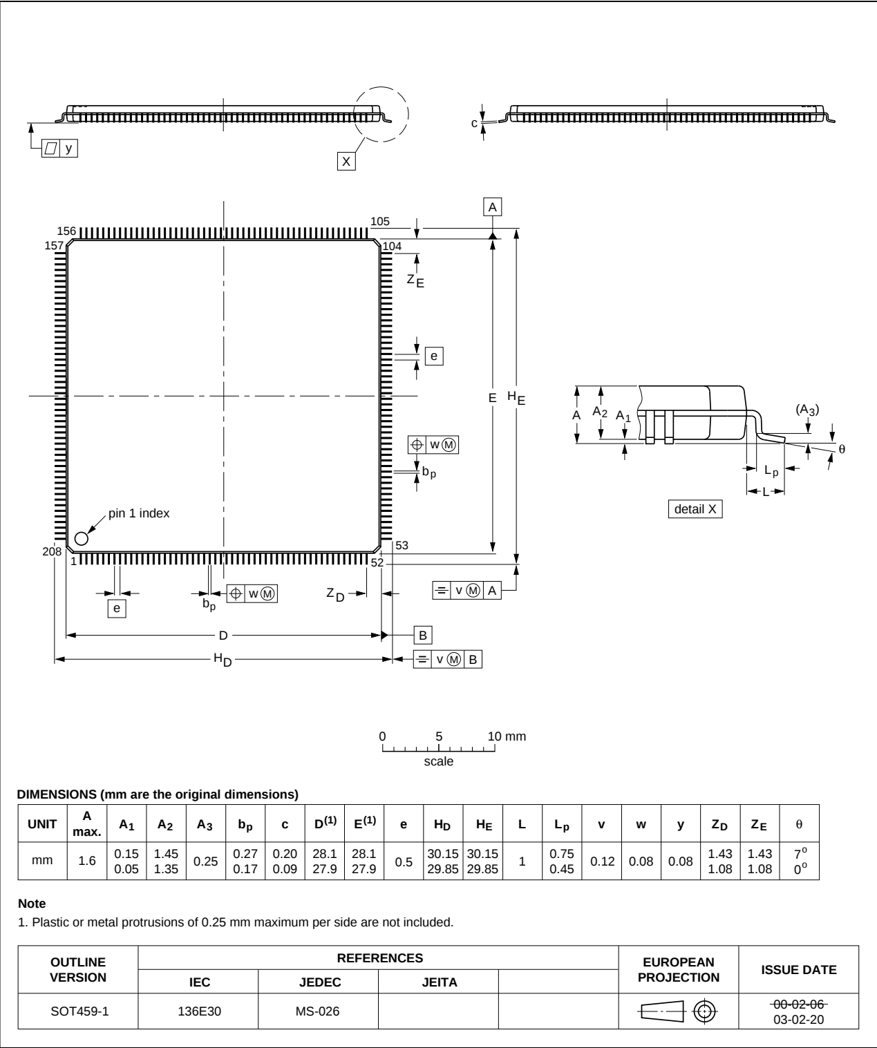
Fig 41. LQFP208 package
