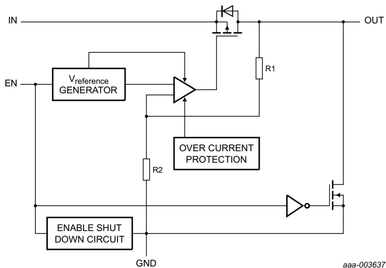
Fig 2. Block diagram of LD6805K/xxP (auto discharge function)
