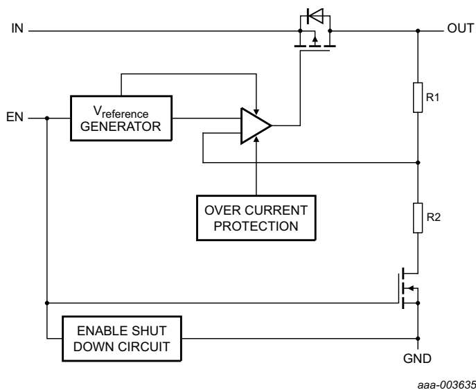
Fig 3. Block diagram of LD6805K/xxH
