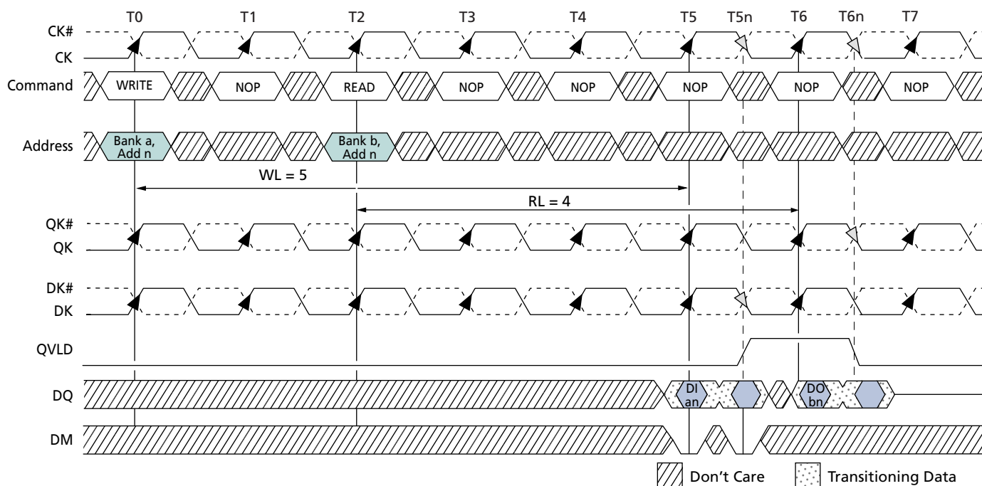
Figure 44: WRITE-to-READ
