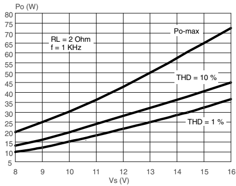
Figure 4. Output Power vs. Supply Voltage (2 \Omega )
