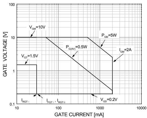
Figure 3. Gate Characteristics
