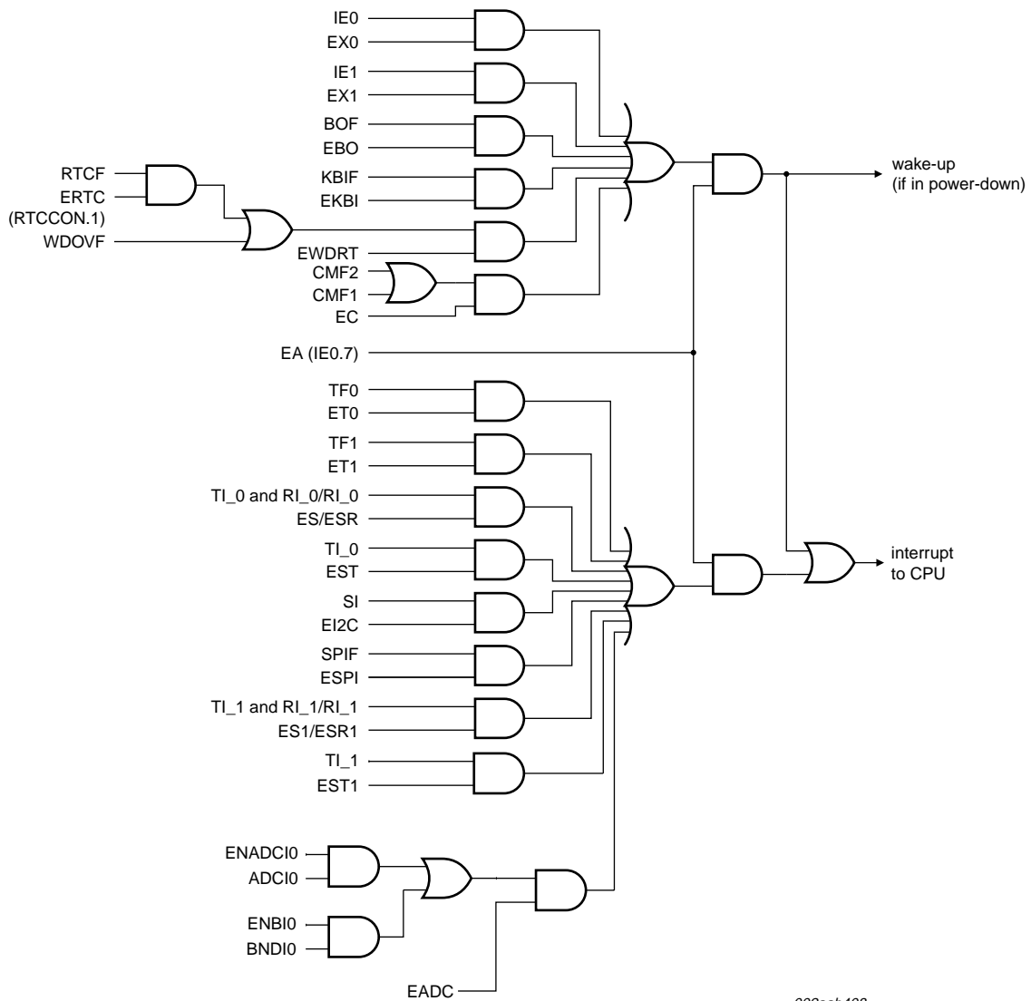
Fig 12. Interrupt sources, interrupt enables, and power-down wake-up sources
