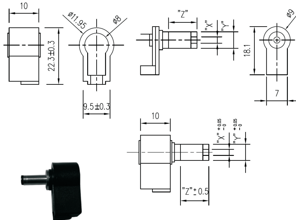
DC PLUG (RIGHT ANGLE TYPE)
