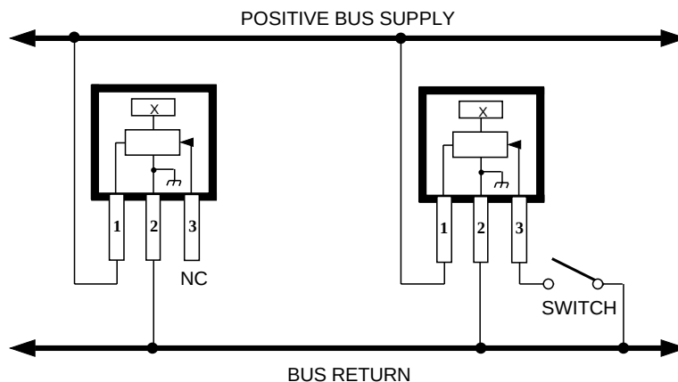
FIGURE 2 SENSOR CONNECTIONS
