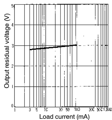
TL-N□MD DC 2-wire Models
