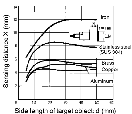
TL-N12MD DC 2-wire Models
