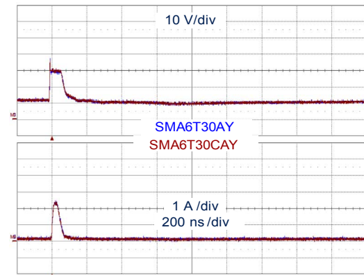
Figure 16. ISO7637-2 pulse 3b: V_s = +150\text{ V} with 12 V battery
