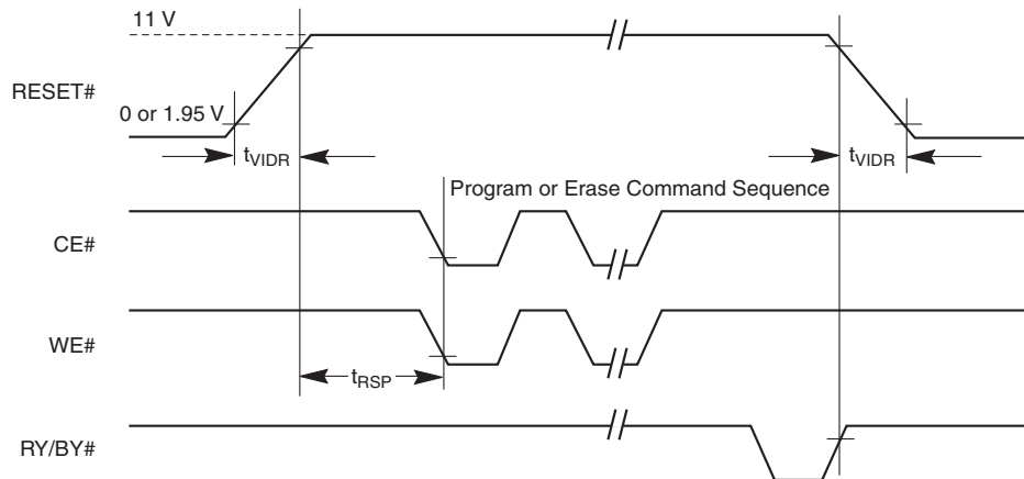
Figure 18.10 Temporary Sector Group Unprotect/Timing Diagram
