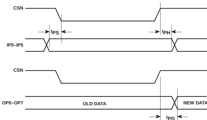
Figure 7. Port Timing
