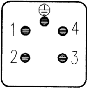
Contact arrangement
