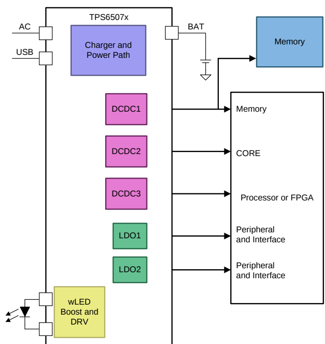
Block Diagram
